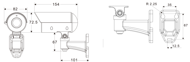
Dimension
