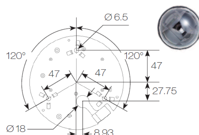
Diagram of mounting holes (unit in mm):
