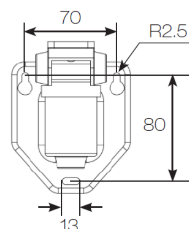
Diagram of mounting holes:
