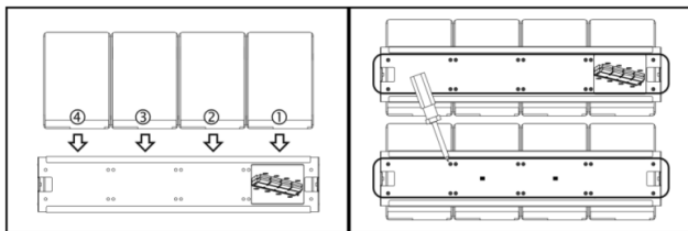
Screws loosened
