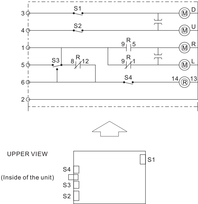
Figure 6 Interconnection Diagram, PIH-302
