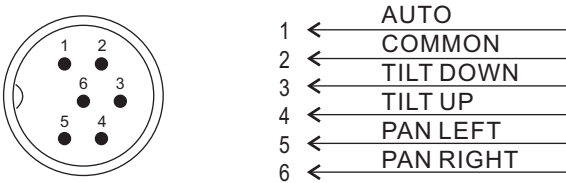
Figure 4 Interconnection Diagram, PIH-302C Control
