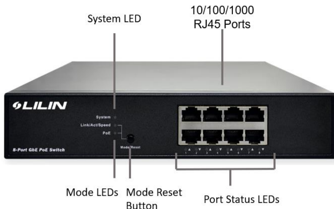
Figure 1: Front panel of the switch
