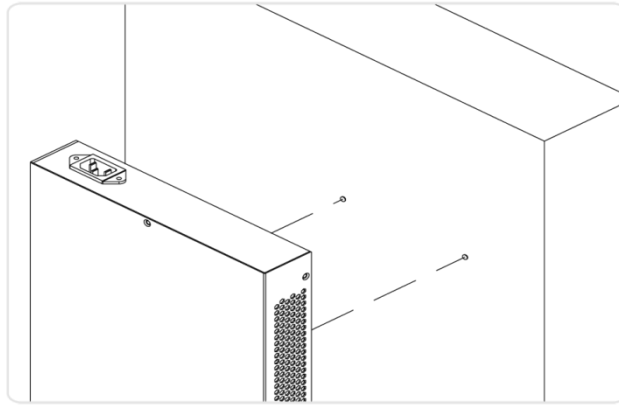
Figure 4: Attaching switch to the wall
