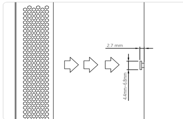
Figure 3: Install screws to the wall
